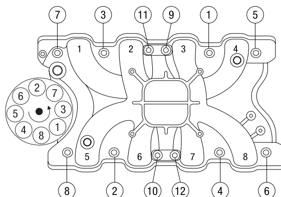
Figure 3 - 351-M/400 Ford Torque Sequence Torque Bolts to 25 ft/lbs.
