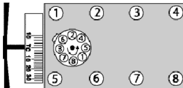
Figure 2 - 289-302 c.i.d. Ford V8
