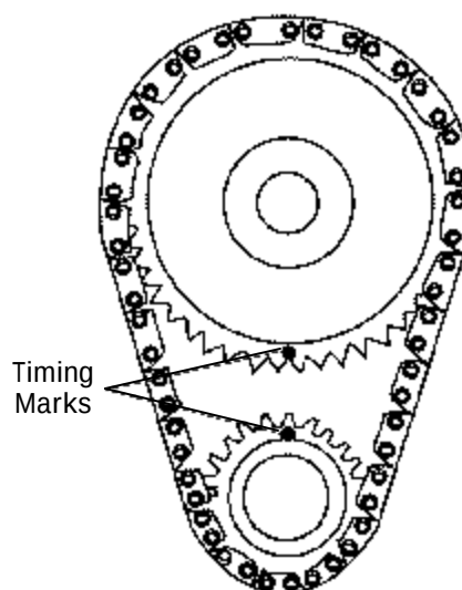
Figure 1 - Timing Chain Sprocket Alignment.
