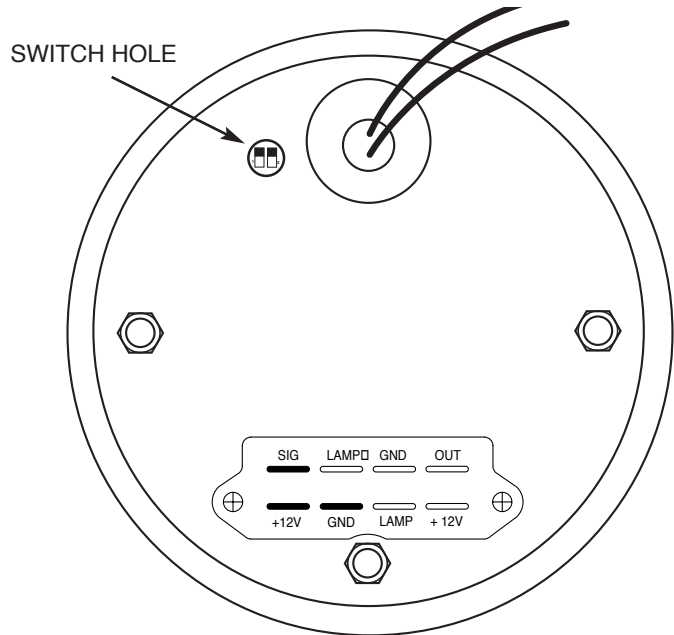
3 3/8" SIZE SHOWN
