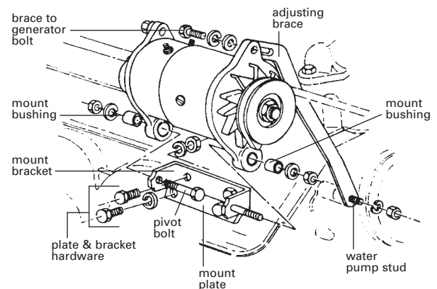
H 58-62 Generator Mount
