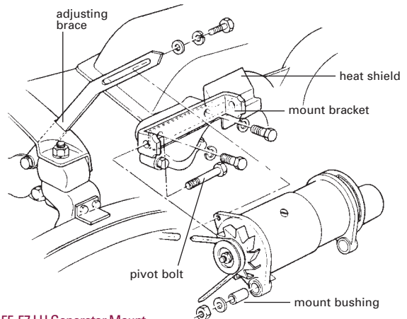
G 55-57 LH Generator Mount
