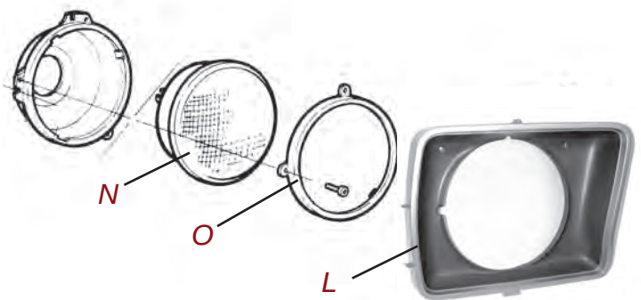
1973-79 HEADLIGHT (Round Type)
